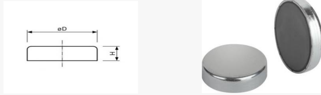
Size specification of ferrite flat shallow pot magnet
